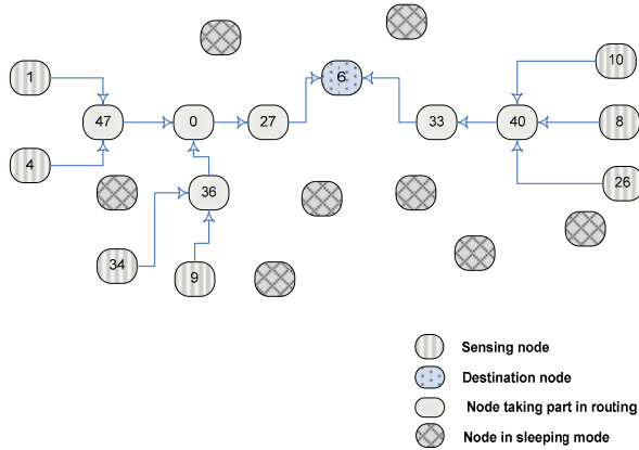
Figure 2. A many-to-one routing scenario where several sensor nodes sense an event at any given moment and try to route the sensory data using the shortest path to the sink.
