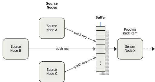
Figure 4. Buffer management scheme for servicing route-thru packets
